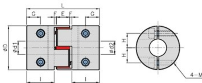
TYPE: SRJ-40C-RD ~ SRJ-80C-RD
