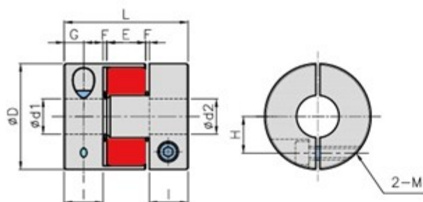
TYPE: SRJ-20C-RD ~ SRJ-30C-RD
